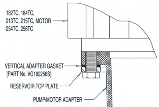
Vertical Mounting Information for 182TC, 184TC, 213TC, 215TC, 254TC, 256TC Motors
