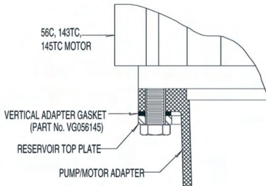
Vertical Mounting Information for 56C, 143TC and 145TC Motors
