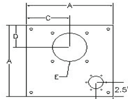
TVL-937A c/w Filler Cutout Motor Adaptor Cutout Adaptor Style 1
