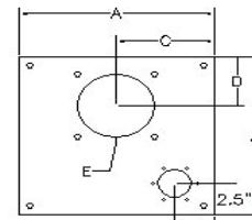
TVL-926 c/w Filler Cutout Motor Adaptor Cutout adaptor Style 1,1A,1B
