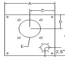
TVL-929A c/w Filler Cutout Motor Adaptor Cutout Adaptor Style 7
